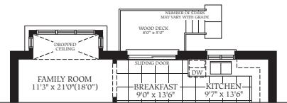
GROUND FLOOR WALK-OUT DECK CONDITION
