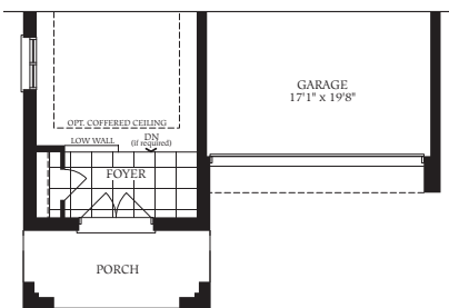
GROUND FLOOR ELEVATION A
