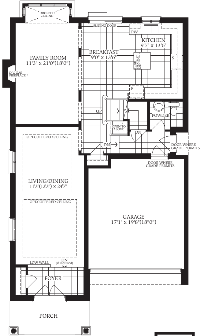
GROUND FLOOR ELEVATION B
